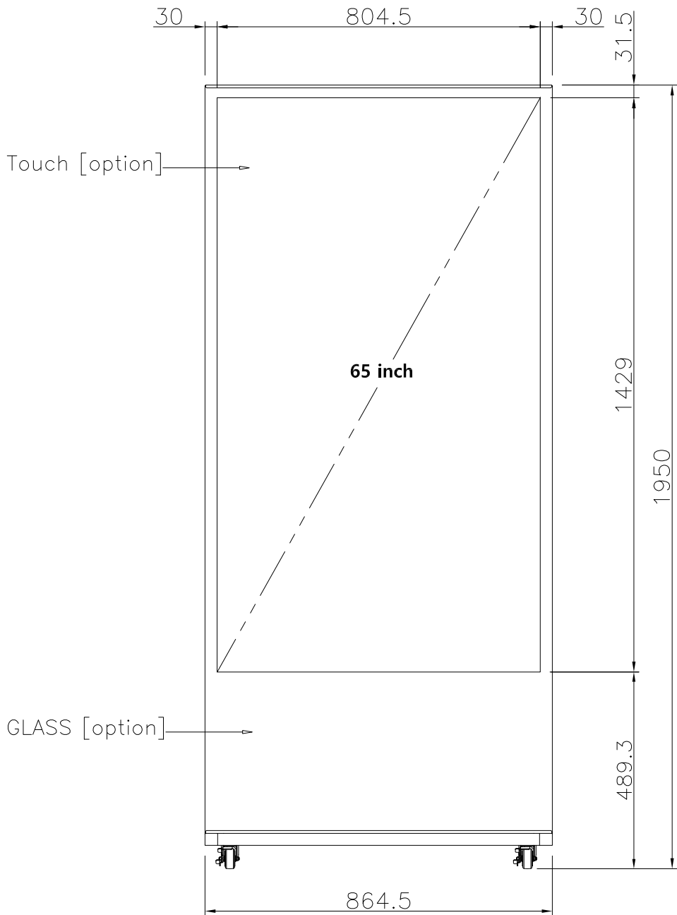
FRONT VIEW
