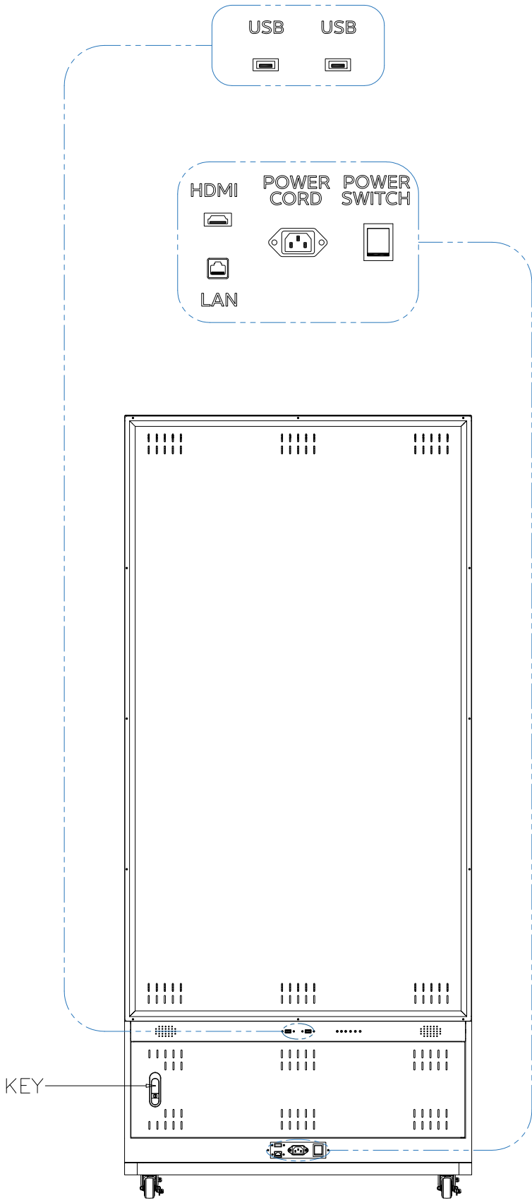
REAR VIEW
